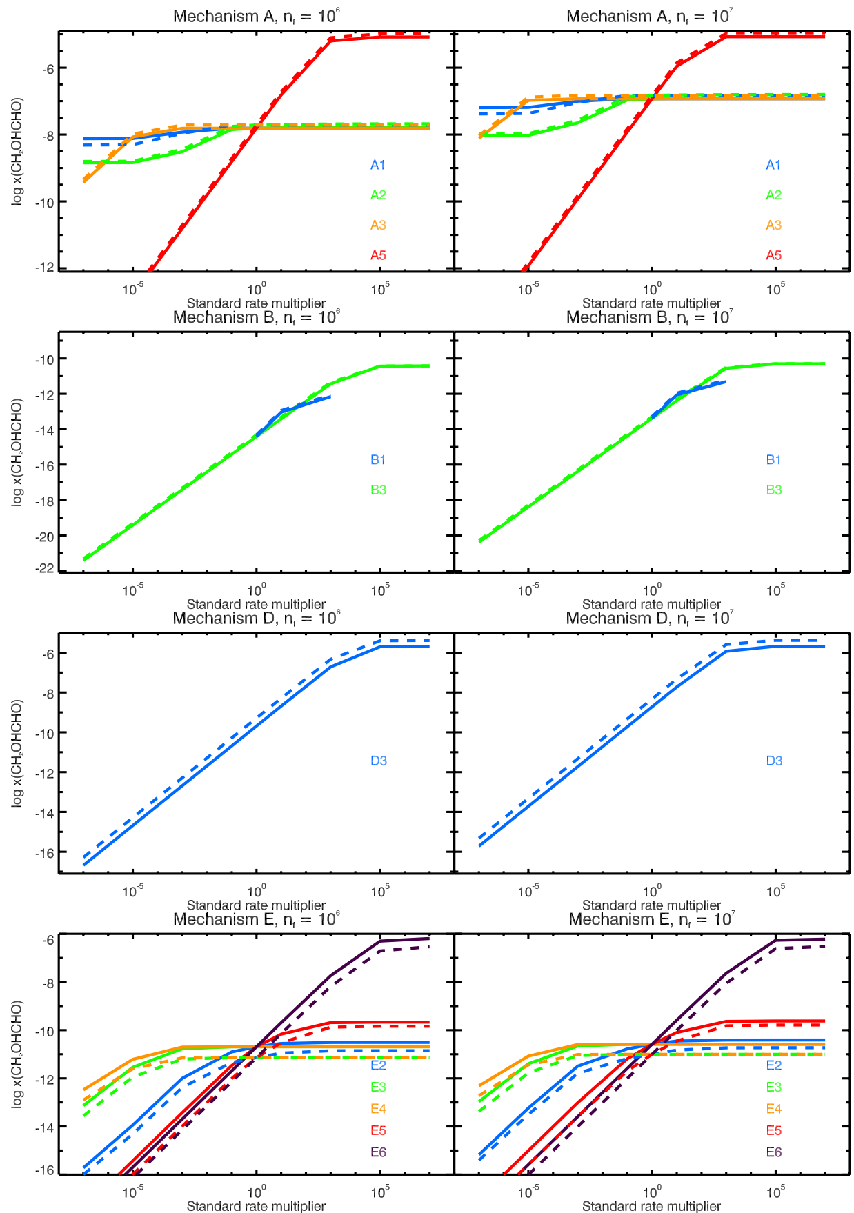
Figure 2. Production of glycolaldehyde via mechanisms A, B, D, and E, for n_f = 10^6 and 10^7 \text{cm}^{-3} (see Section 4.4 for a description of mechanism C). The solid lines show results using hydrogenation regime f1; the dashed lines, regime f2. Standard rates can be found in Table 3.
